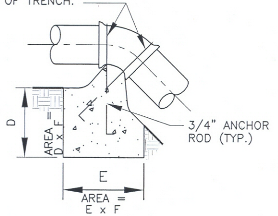
VERTICAL BEND
