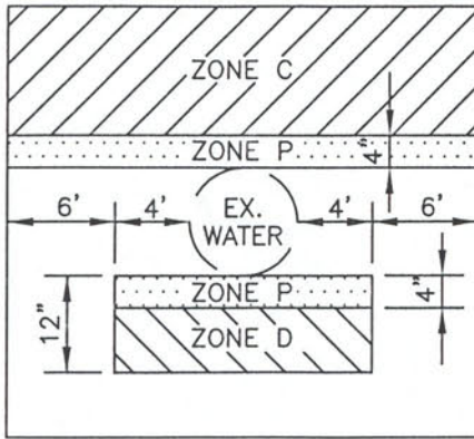
PERPENDICULAR CONSTRUCTION
