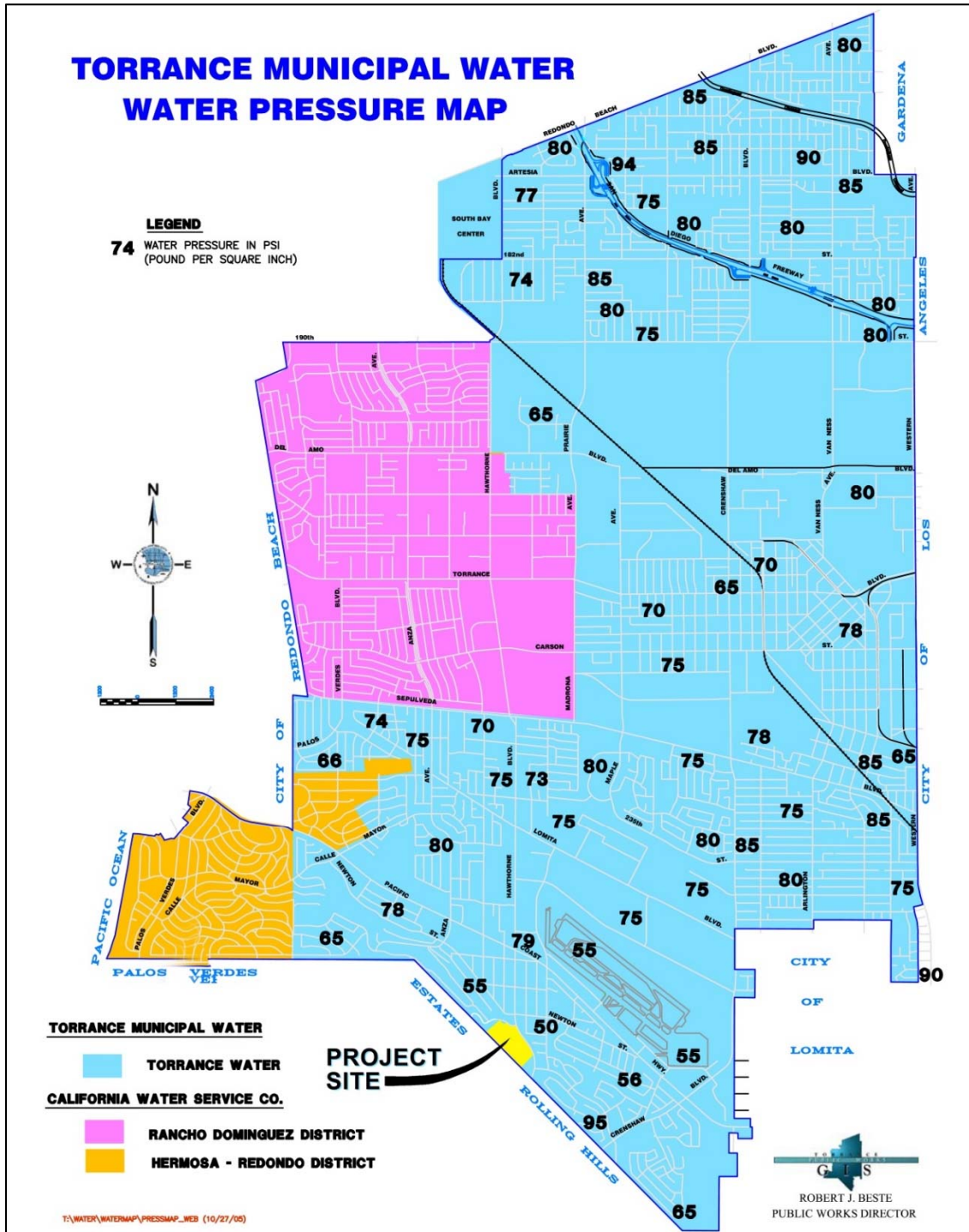
Figure 5 – Water Pressure Zones
