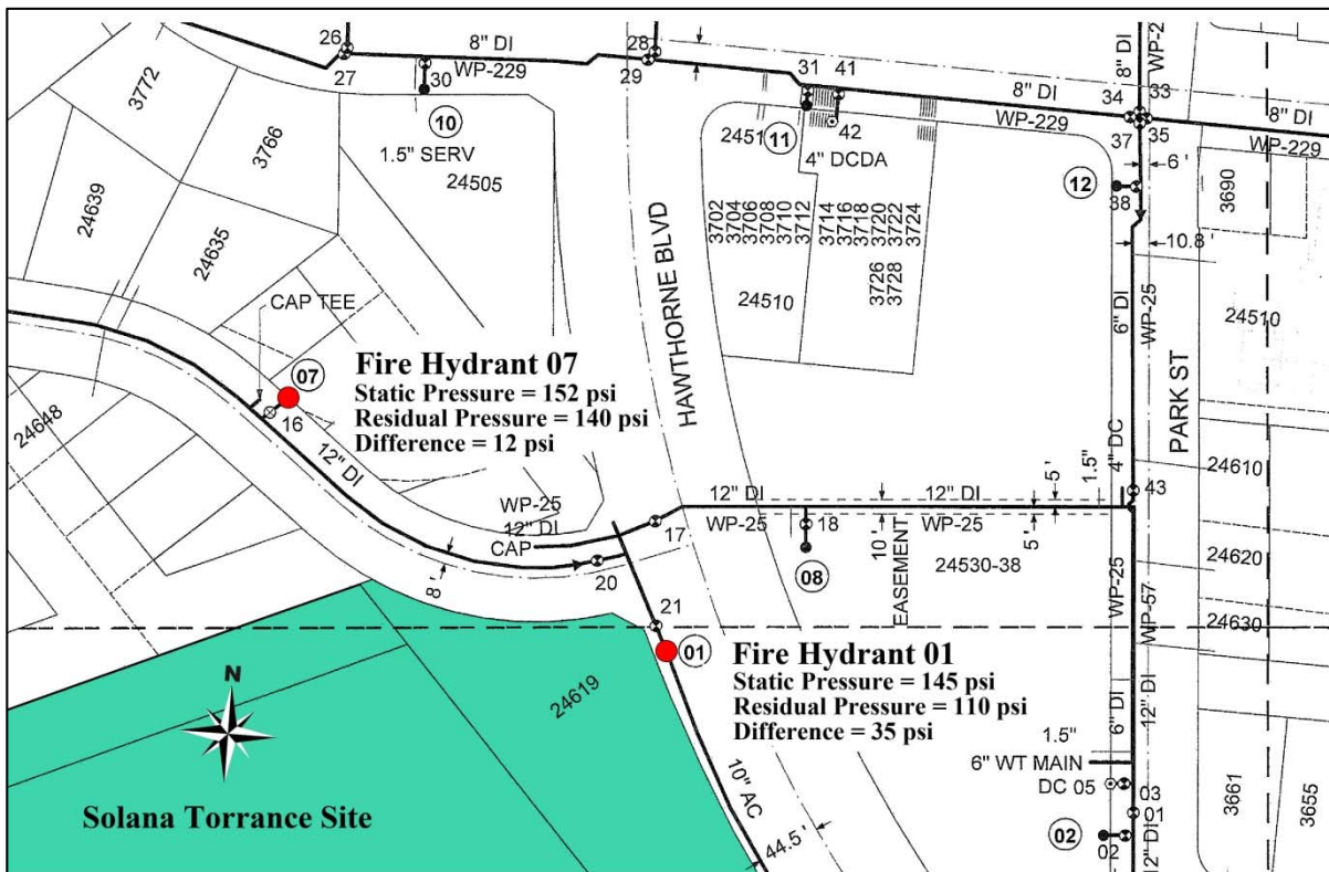
Figure 6 – Fire Flow Test Fire Hydrant Locations
